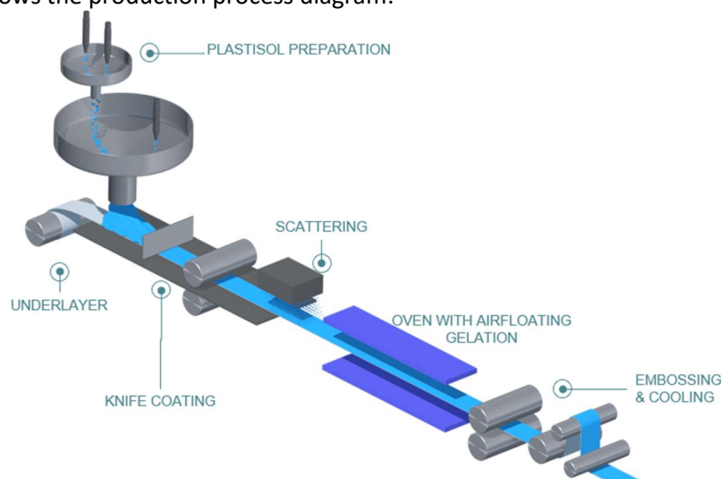
Figure 1: Coating process
